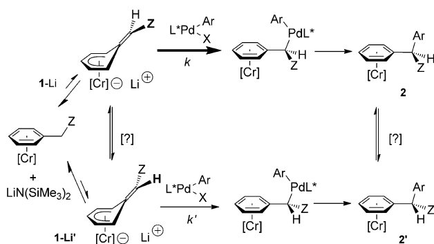
Scheme 3. Proposed asymmetric arylation of tricarbonylchromium-stabilized benzyllithiums showing the reversible deprotonation and inter-conversion of lithiated enantiomers, enantiodetermining transmetalation to palladium, and reductive elimination to form 2 .
